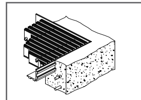
76mm grating: PN# 1618005 Install 76mm side vertical
