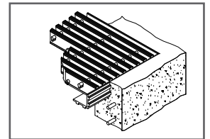
64mm grating: PN# 1618005 Install 64mm side vertical
